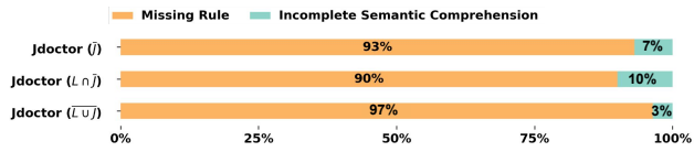
(b) Root causes of the baseline method (Jdoctor)
